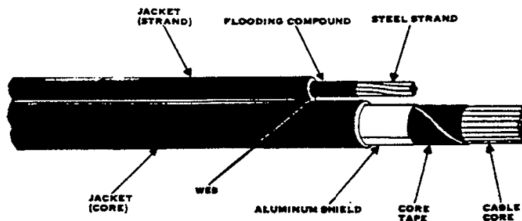
Figure 9 – Alpeth-FPA Cable
