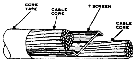
Figure 2 – Alpeth-FPA-T Screen Cable
