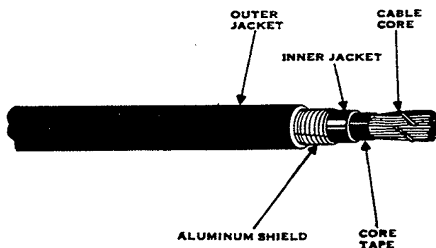
Figure 11 – DS Alpeth-FPA Cable
