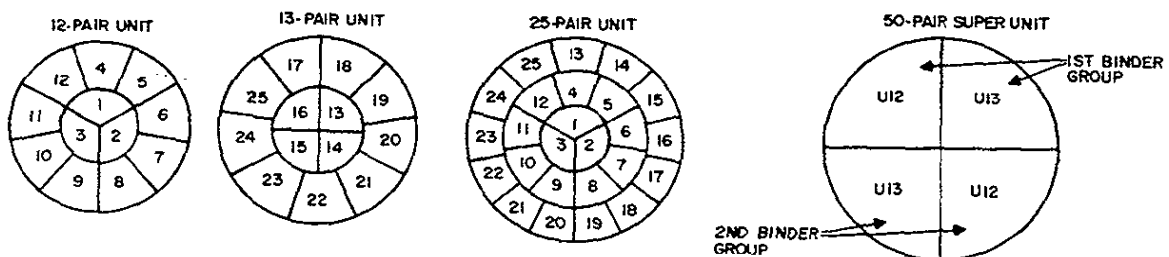
Figure 24 – Unit Arrangement, Alvyn Cable
