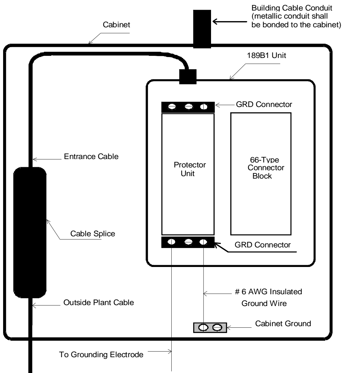
Figure 7: Typical Bonding and Grounding at Cable Entrance (OSP Cable)
