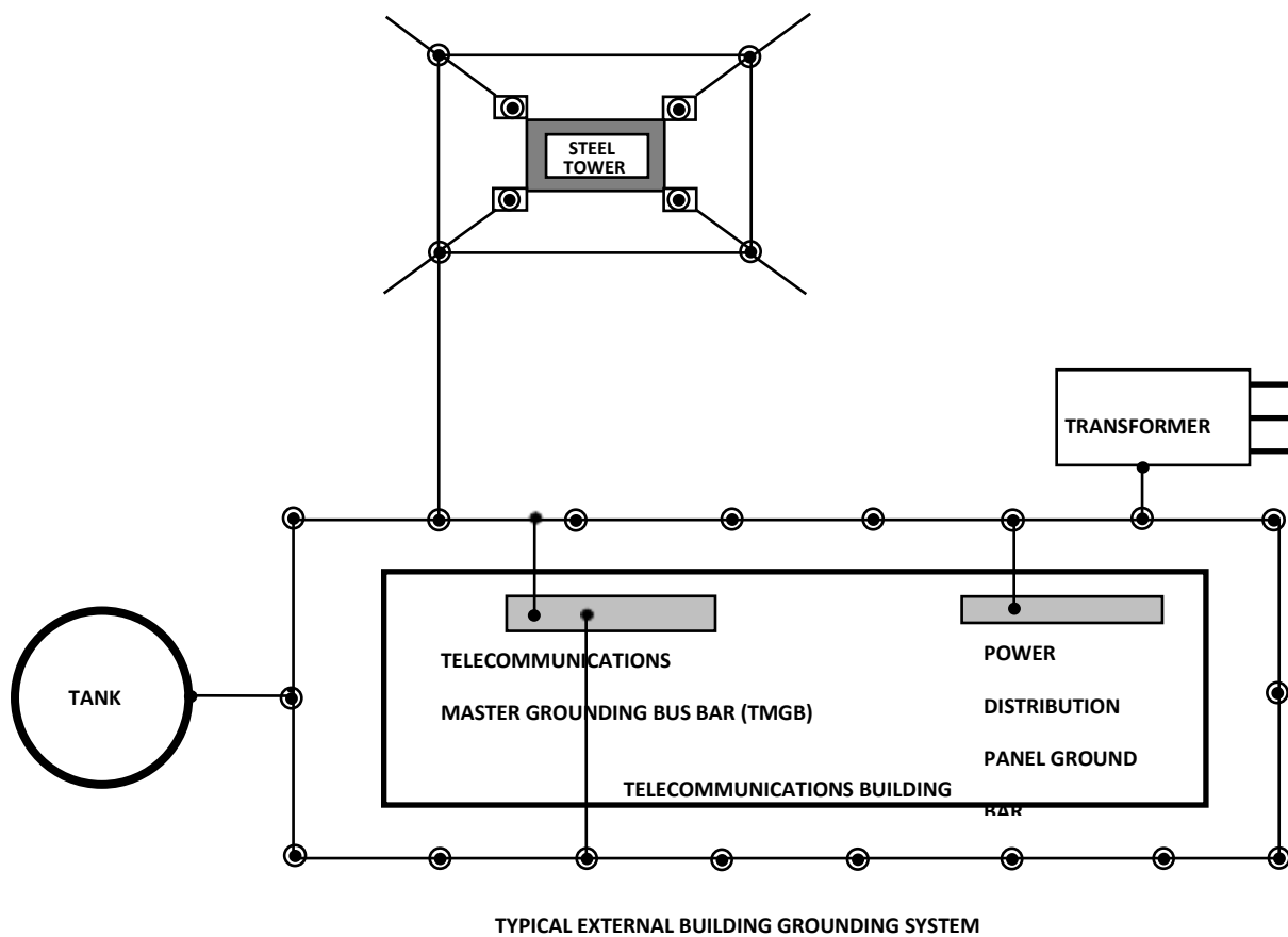
Figure 3: Typical External Grounding System Arrangement
